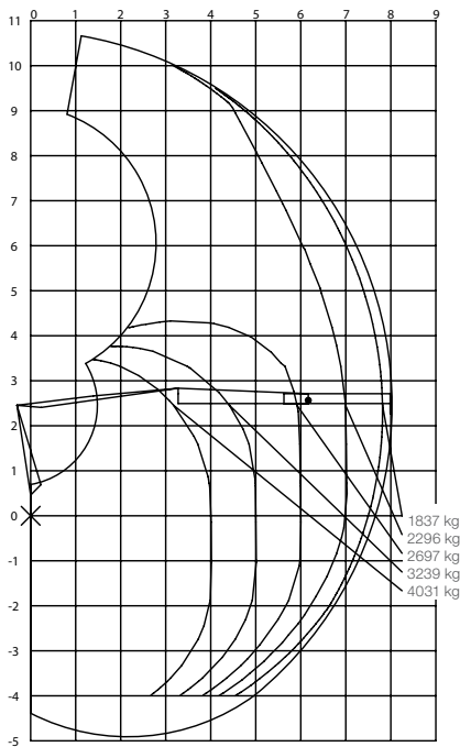
Load diagram J1620Z80
