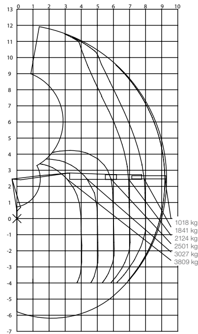
Load diagram J1620Z93
